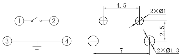
CIRCUIT DIAGRAM
