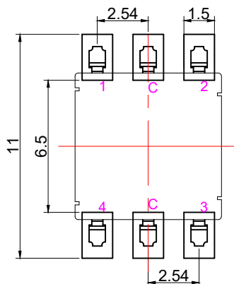
PCB LAYOUT
